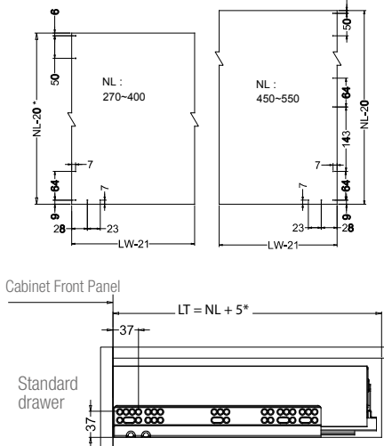
Drawer bottom (Pre-drilling not necessary)
