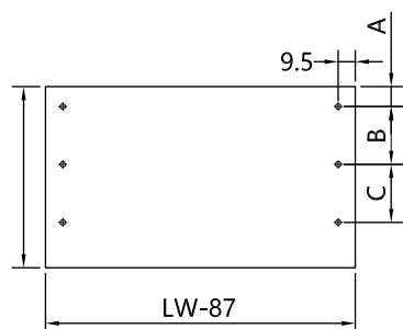
Drawer back (Pre-drilling not necessary)
