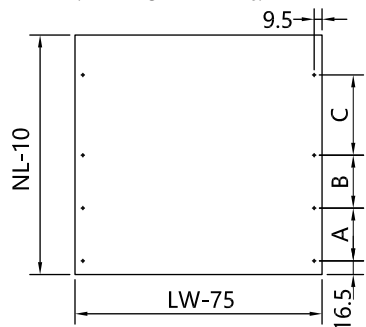
Drawer bottom (Pre-drilling not necessary)
