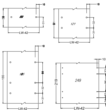
Drawer back (Pre-drilling not necessary)
