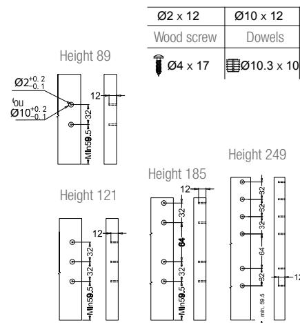
Drawer front drilling (mm)
